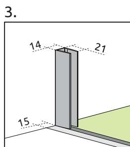
Wariant LEWY Variant L
